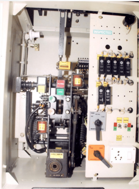
Operating Mechanism 33KV
