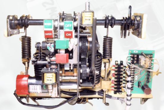
Operating Mechanism 11 KV
