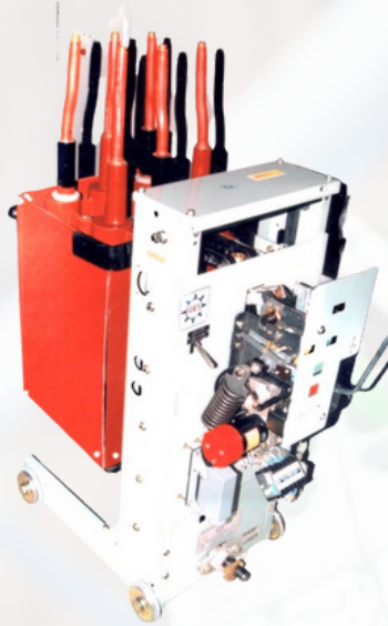
Retrofitting VCB Suitable for Crompton Greaves
